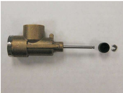
Complete Valve Repair Kit 200851484
