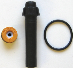
repair kit 200457180 for ST-457 Turbo Nozzle 8.0
